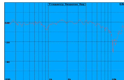
Frequency response 200 Hz to 20 kHz at 30°
