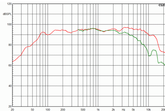
Frequency response in 1/3 octaves, dBspl/1m/2.83V at 0° and 30°
